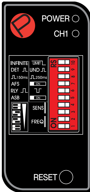
Figure 3. LC20-1 Faceplate
